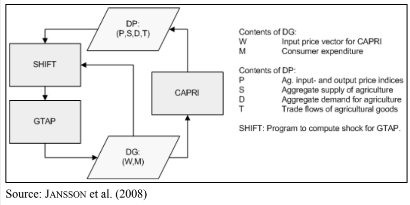
Figure 1. CAPRI-GTAP linkage
