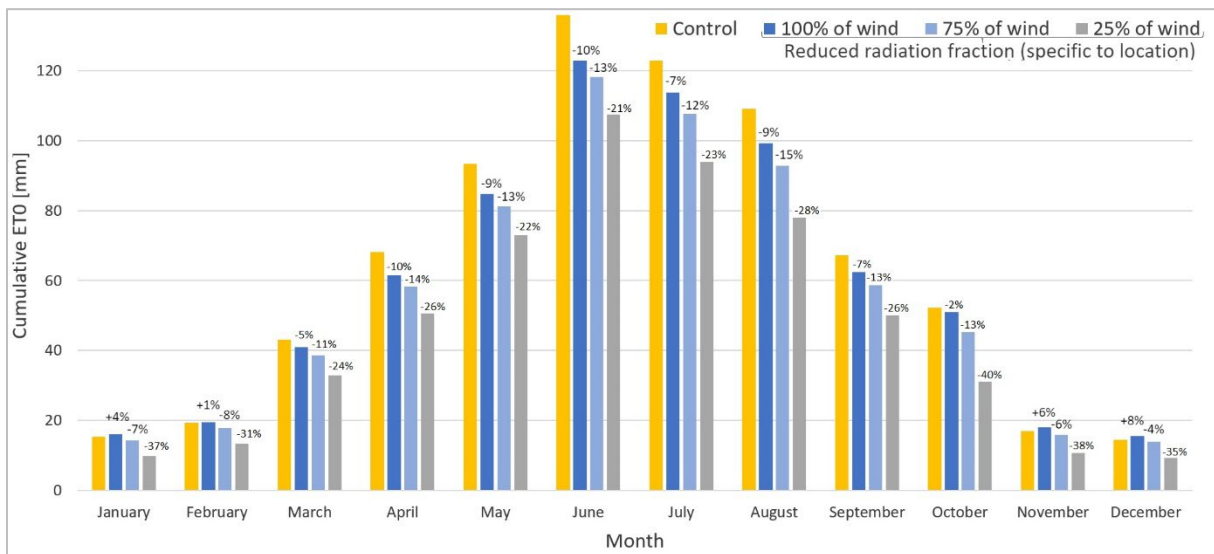
Figure 7. Cumulative ET0 along year 2005 in central France at Channay (percentages overhead the bars are the relative difference with the control scenario).
