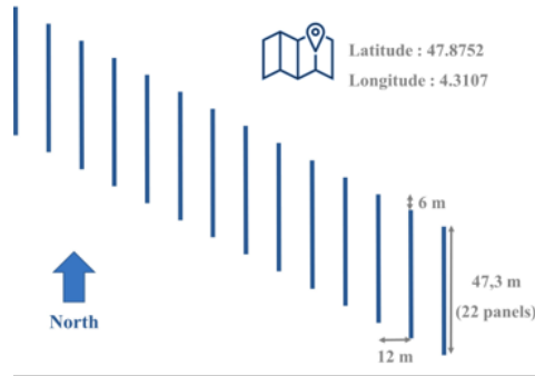
Figure 3. Aerial view diagram of the studied configuration.
